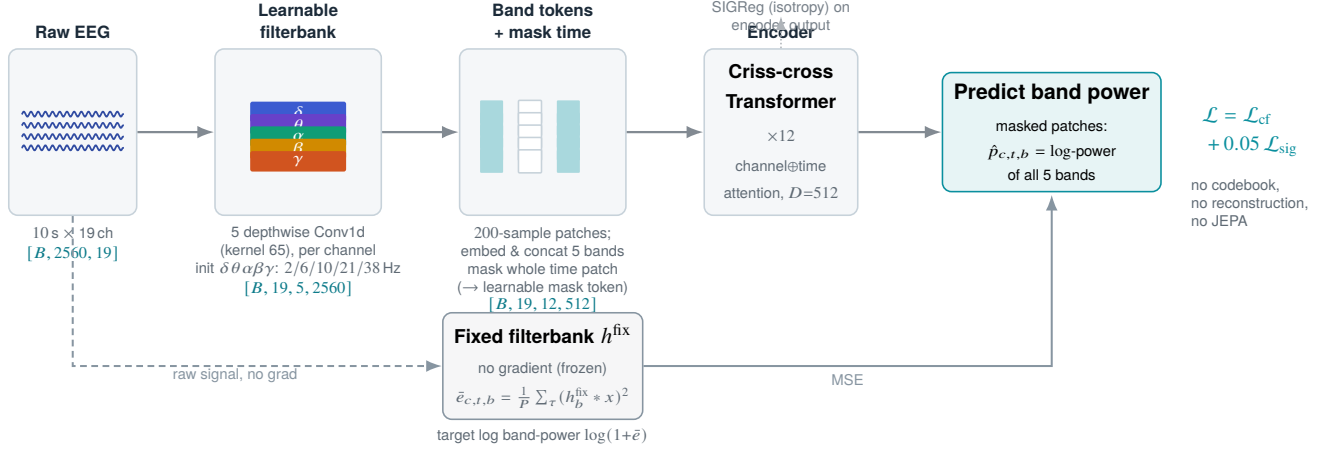
Figure 2: Codebook-free spectral-prediction pretraining. A learnable filterbank tokenizer splits each patch into \delta\theta\alpha\beta\gamma bands; time patches are masked out of the encoder input. From the encoder output the model regresses the log band-power of masked patches, supervised by a fixed , non-learnable filterbank target that cannot be collapsed; SIGReg adds an isotropy penalty. (A raw-signal reconstruction head we included is inert on this tokenizer—its loss stays zero—so the effective objective is purely spectral.)
