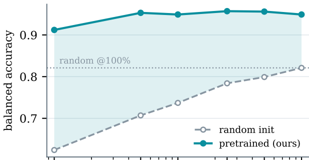
ISRUC (seq2seq head)
