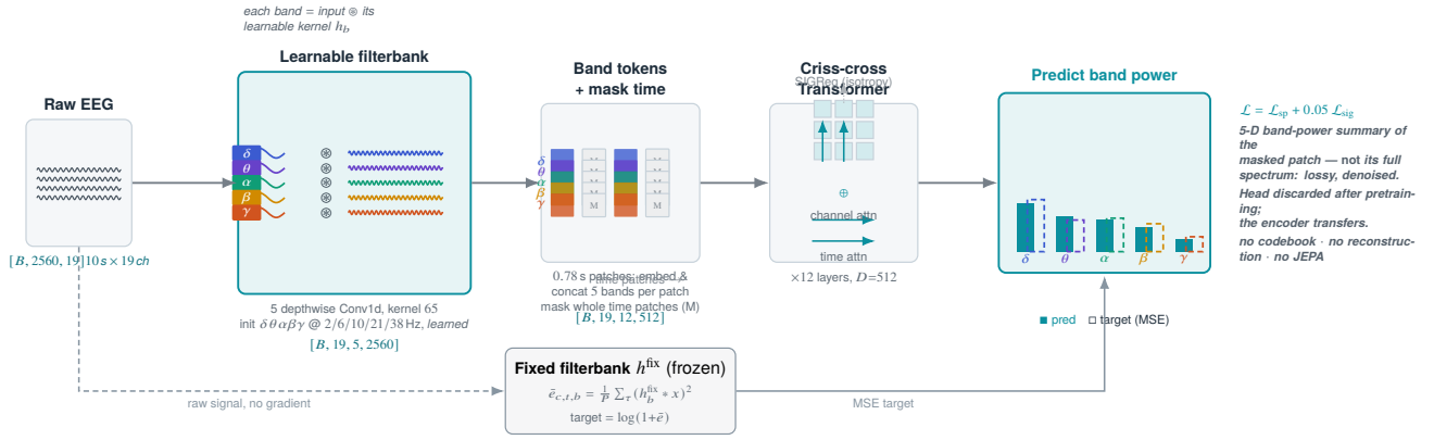
Figure 2: Codebook-free spectral-prediction pretraining. A learnable filterbank tokenizer splits each patch into \delta\theta\alpha\beta\gamma bands; time patches are masked out of the encoder input. From the encoder output the model regresses the log band-power of masked patches, supervised by a fixed , non-learnable filterbank target that cannot be collapsed; SIGReg adds an isotropy penalty. There is no reconstruction, discrete-codebook, or latent term—the objective is purely spectral.
