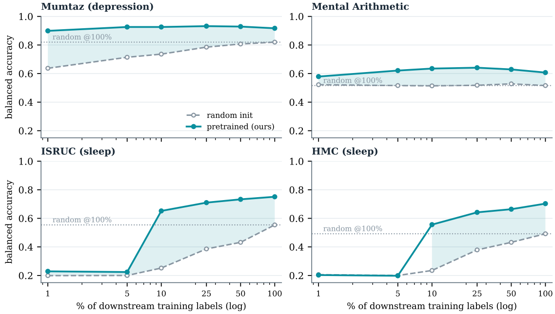
Figure 3: Label efficiency of the ~2,500-hour model. Balanced accuracy of a probe trained on a fraction of downstream labels, pretrained (ours, solid) vs. random init (dashed); dotted line is random at 100% labels, shaded band is the pretrained–random gap. A small fraction of labels with pretraining exceeds all labels without it on every task; on the sequence tasks (ISRUC, HMC) the advantage appears once \geq 10\% of sequences suffice to fit the head.
