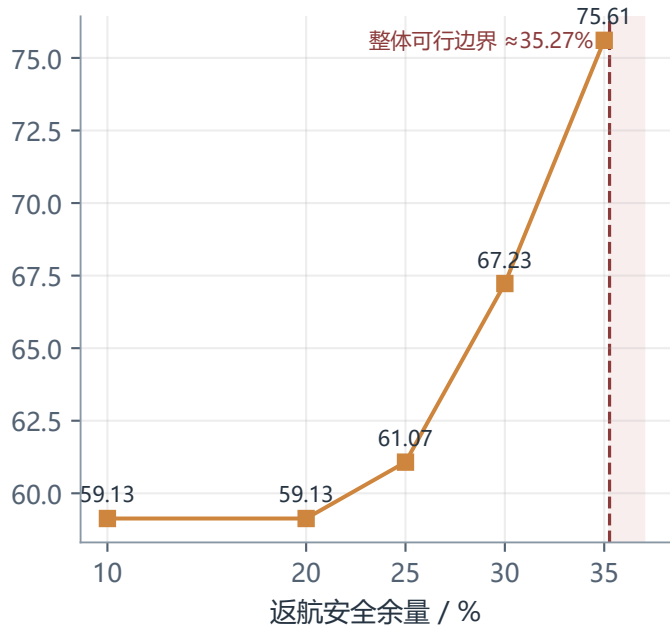
总能耗 / kWh
