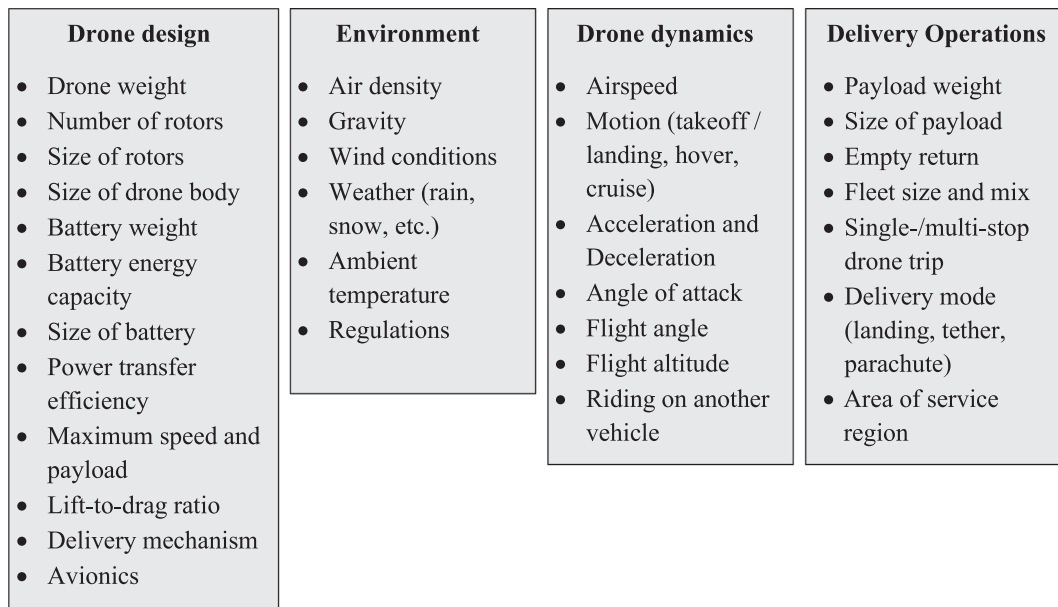
Fig. 1. Factors affecting drone energy consumption.
