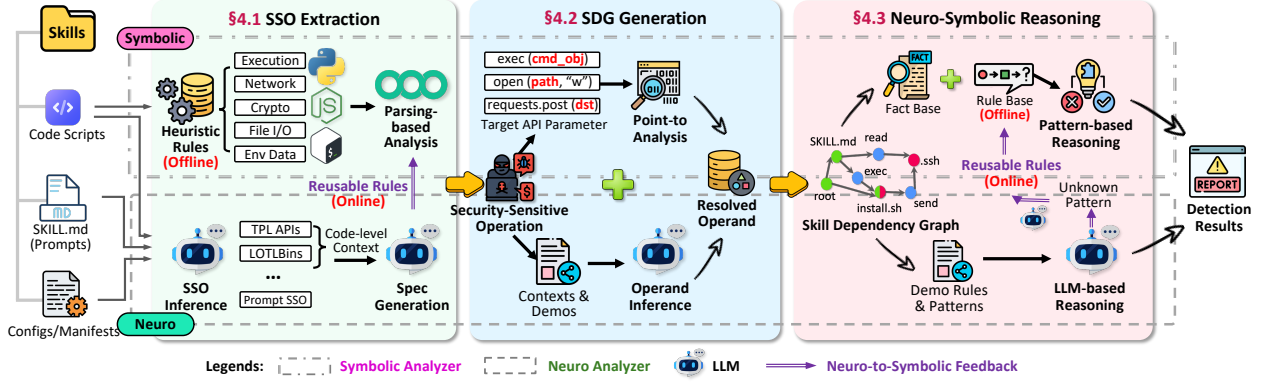
Figure 3: The overall workflow of MALSKILLS.
