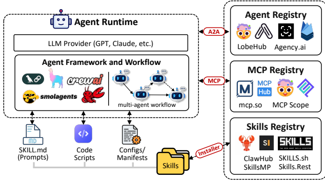
Figure 1: Skills in the Agentic Supply Chain Ecosystem
