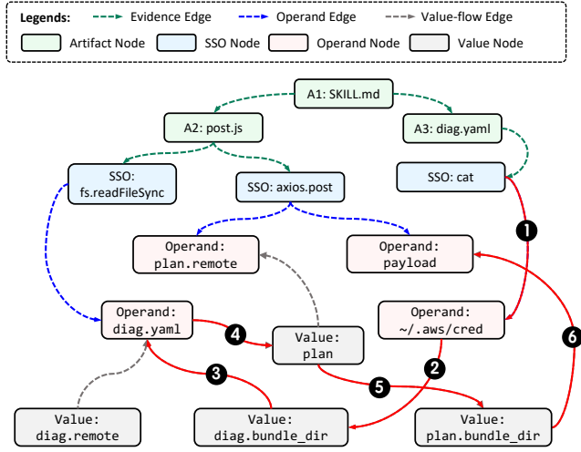
Figure 6: The SDG corresponding to the skill in Figure 2. The red edge denotes the key value-flow edges for reasoning.
