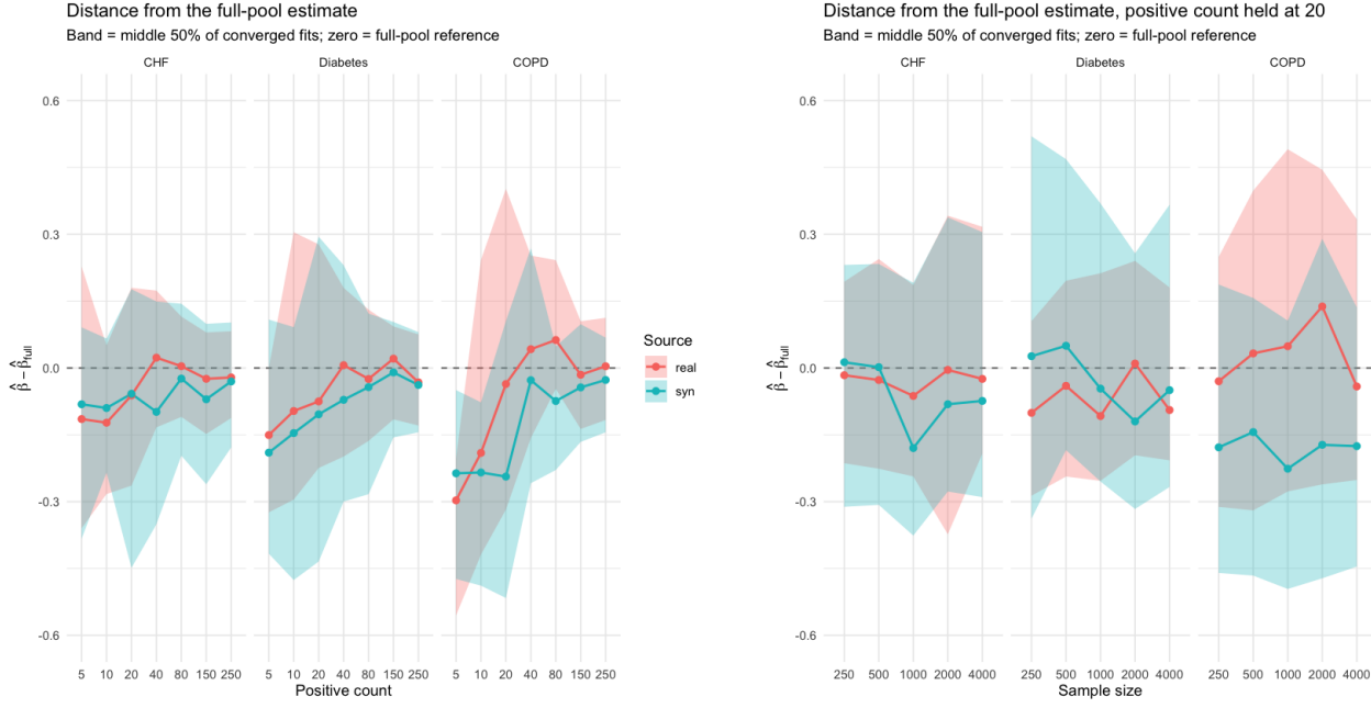
Figure 2: The count narrows the spread (left) and the sample size does not (right), on a common scale. Distance from \hat{\beta}_{full} ; band is the middle 50% of converged fits.
