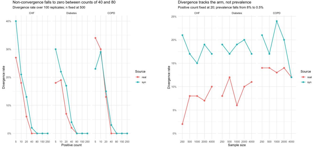
Figure 1: Divergence falls away under the count (left) and not under the sample size (right); note the differing vertical scales. The two smallest counts are detection floors.
