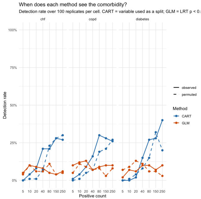
Figure 5: The null (dashed) climbs with the count alongside the observed rate (solid), so the rise is not recovery. CART in blue, the matched GLM in orange.
