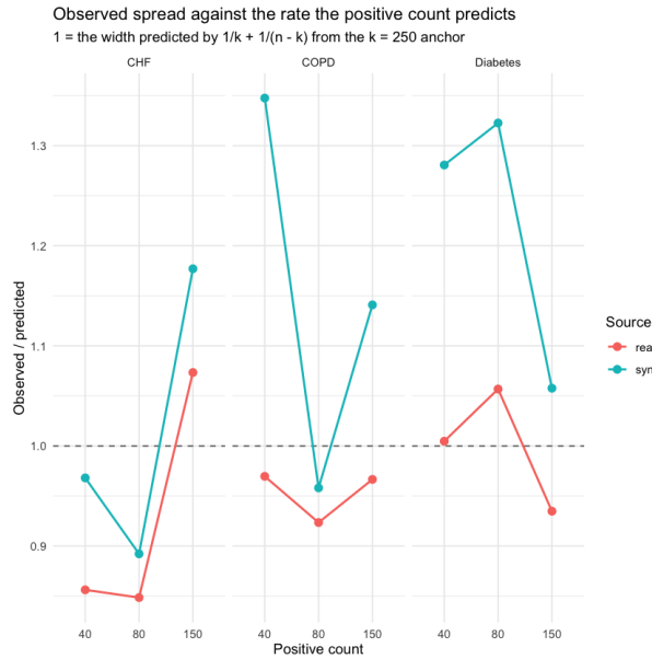
Figure 3: The real arm tracks the width its count predicts; the synthetic arm sits above the real one in all nine matched cells.
