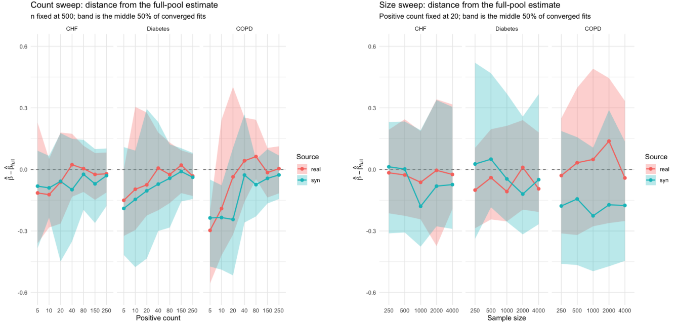
Figure 2: Left, the count sweep: the spread narrows. Right, the size sweep: it does not. Common scale, plotted as distance from \hat{\beta}_{full} ; band is the middle 50% of converged fits.
