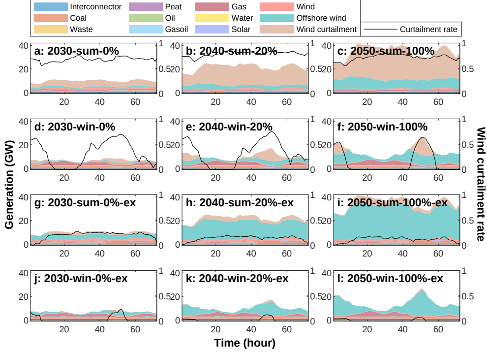
Fig. 4 Power system operation results. Different years, seasons, hydrogen blending ratios and export conditions are compared. 2030, 2040 and 2050 indicate the model year; sum and win indicate a typical summer day (high wind and low demand) and a typical winter day (low wind and high demand), respectively; 0%, 20% and 100% indicate different maximum allowed hydrogen blending potentials; ex indicates export access.
