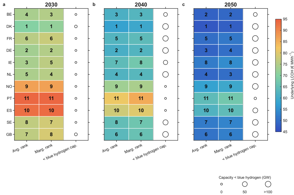
Fig. 3 Country rankings for offshore green hydrogen cost competitiveness. a–c, Cost-competitiveness metrics for 2030, 2040 and 2050, respectively. Cell numbers report average and marginal LCOH ranks among the 11 countries, and colours show the underlying LCOH values. Marginal LCOH is evaluated at each country’s offshore wind capacity target, whereas average LCOH is calculated across the national cost-supply curve. Circles show the hydrogen production capacity with LCOH below the upper bound of the blue-hydrogen benchmark; the smallest and largest circles denote 0 and \geq 100 GW, respectively.
