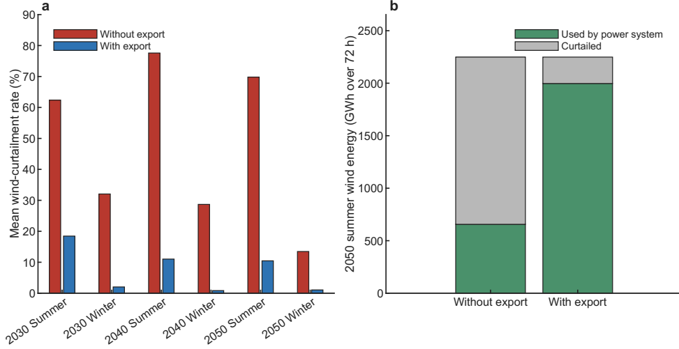
Fig. 3 Export access reduces domestic wind curtailment in the Ireland power-gas case. a Mean wind-curtailment rates across representative summer and winter periods in 2030, 2040 and 2050, with and without export access. b Decomposition of available wind energy in the 2050 summer representative period. Export access converts otherwise curtailed wind into energy used by the power system, but residual curtailment remains because operating constraints still bind at the margin.
