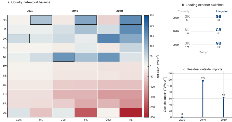
Fig. 5 Lowest-LCOH allocation misidentifies strategic offshore hydrogen exporters. a Country net-export balance under a lowest-LCOH-only baseline and the integrated model in 2030, 2040 and 2050. Blue indicates net export and red indicates net import. Black boxes mark the leading net exporter in each model-year combination. b Leading net exporter and corresponding net export under the two model structures. c Residual outside imports identified by the integrated model. The cost-only baseline allocates demand within the modelled European offshore supply by construction and therefore does not expose the residual external import requirement.
