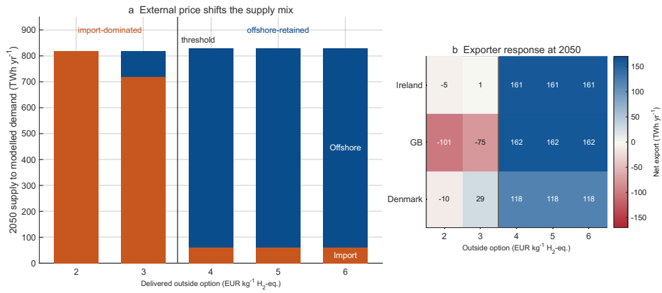
Fig. 7 External import prices define a threshold for European offshore hydrogen supply. a 2050 supply mix between external low-carbon imports and European offshore hydrogen under delivered outside-option prices from 2 to 6 EUR kg -1 H 2 -equivalent. b Net-export response of Ireland, the United Kingdom and Denmark under the same price scan. Blue indicates net export and red indicates net import. The scan is designed to identify a price threshold, not to assign probabilities to future import prices.
