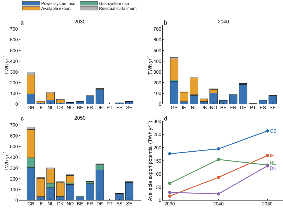
Fig. 4 Domestic absorption creates uneven exportable offshore surplus across Europe. a-c Country-level decomposition of offshore wind use in 2030, 2040 and 2050, ordered by 2050 available export potential. Power-system use, gas-system use, available export potential and residual curtailment are reported in TWh yr -1 . d Export-potential trajectories for the United Kingdom, Ireland, the Netherlands and Denmark.
