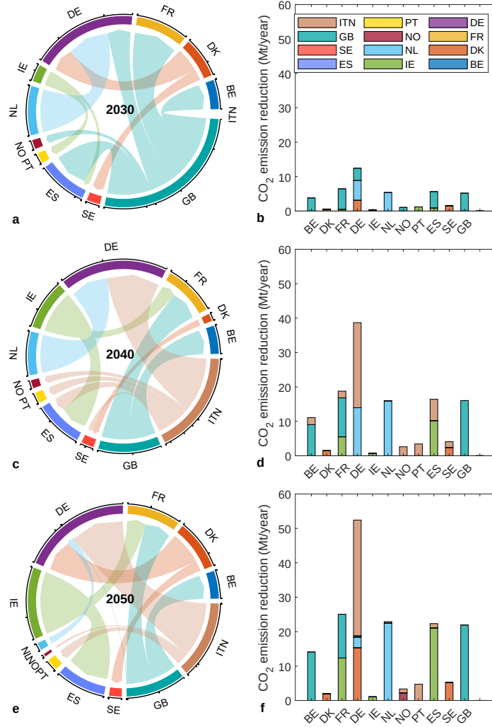
Fig. 6 Sankey diagram of hydrogen flows and contributions to carbon mitigation. a, c, and e, are the Sankey diagrams of hydrogen flows among these countries and external hydrogen imports in 2030, 2040, and 2050, respectively. ITN represents external import. Only the hydrogen flows between countries are drawn; hydrogen supplied and consumed within the same country is not shown. b, d, and f show supplier-attributed carbon mitigation in the optimized supply mix, including domestic self-supply and exports. Different bars represent the reduction in carbon dioxide emissions, and different colours indicate different countries' contributions. ITN contributions are excluded when reporting European offshore supplier contributions.
