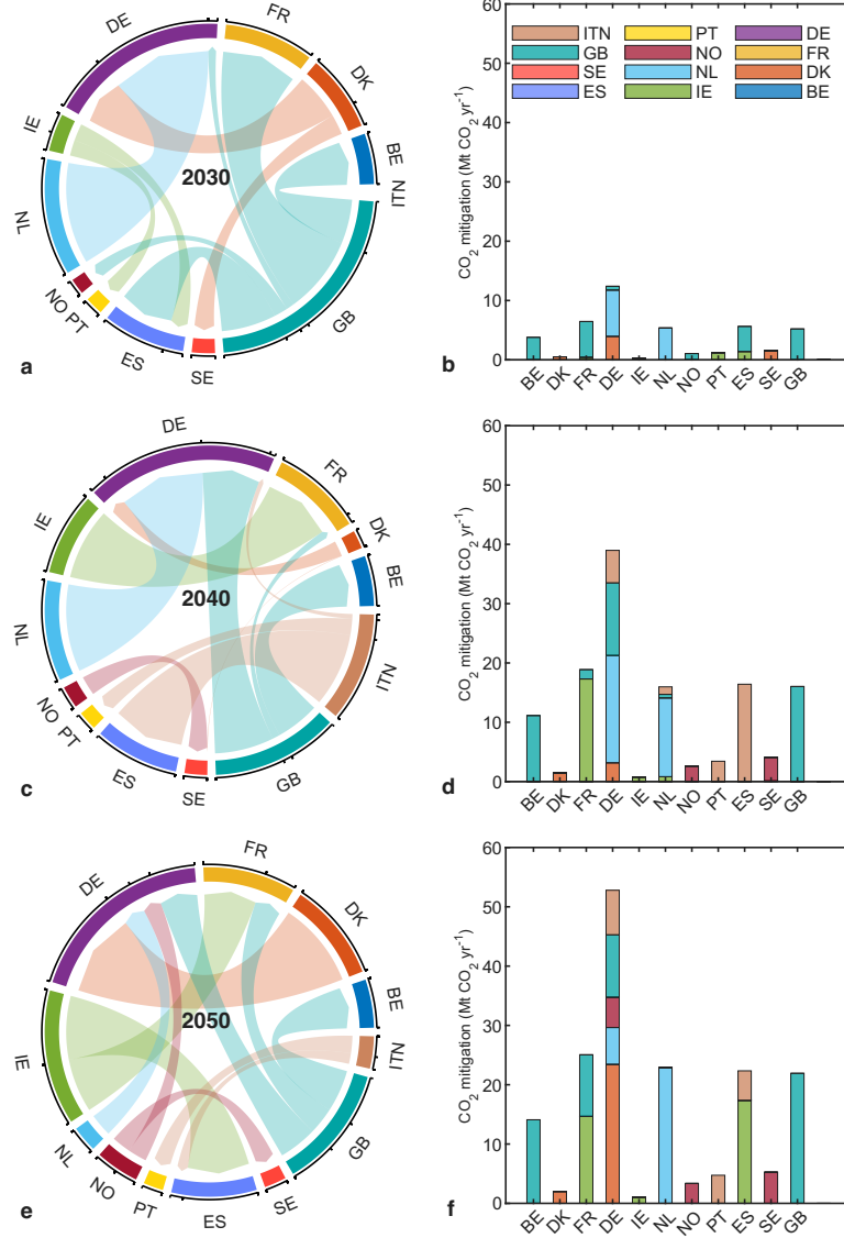
Fig. 6 Hydrogen trade flows and supplier-attributed carbon mitigation. a, c, and e, Cross-border hydrogen flows among European countries and external imports in 2030, 2040 and 2050, respectively. ITN represents external imports. Hydrogen supplied and consumed within the same country is not shown. b, d, and f, Supplier-attributed carbon mitigation in the optimized supply mix, including domestic self-supply and exports. Bar colours identify the supplier contributing the mitigation value. ITN contributions are included in the plotted full supply mix but excluded when reporting European offshore supplier contributions in the text.
