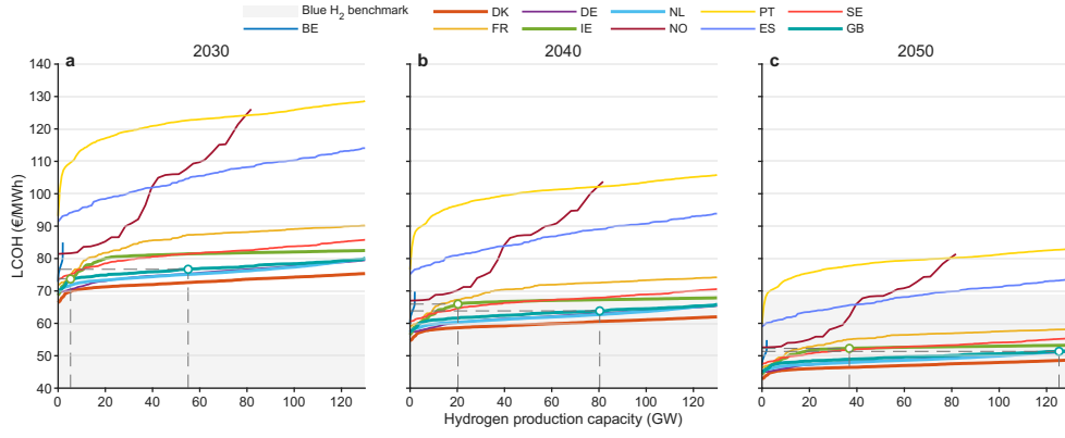
Fig. 2 Cost-supply curves show widening offshore hydrogen competitiveness but do not rank strategic exporters. a–c, Green-hydrogen cost-supply curves for 2030, 2040 and 2050, respectively. Coloured lines show all studied countries; Denmark, Ireland, the Netherlands and the UK are drawn with thicker lines as the main comparisons discussed in the text. Coloured markers denote Ireland’s and the UK’s offshore wind capacity targets on their corresponding supply curves. Grey bands show the assumed future blue-hydrogen production-price range.
