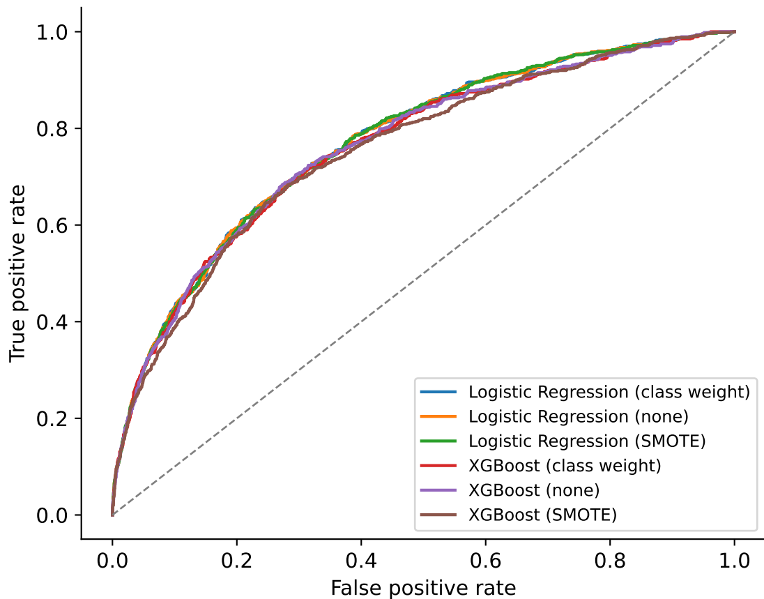
ROC curves on the held-out test set
