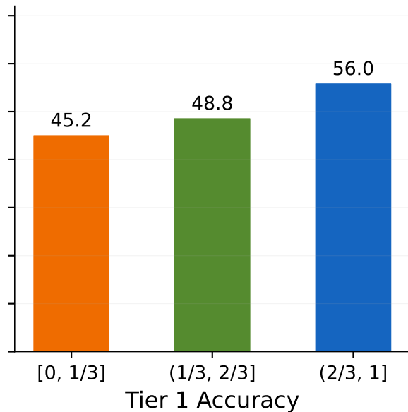
Tier 2 (Pruned)
