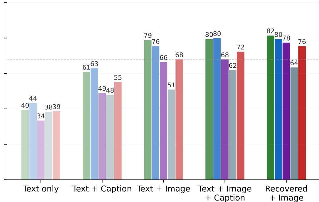
Tier 2 (Pruned)
