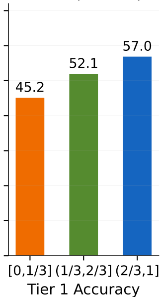
Tier 2 (Pruned)
