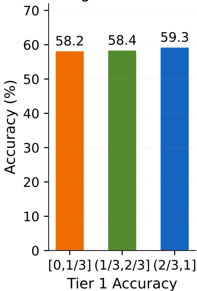
Original Problem
