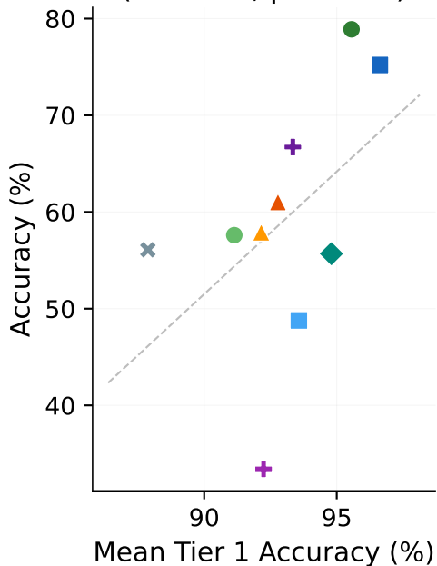
Original Problem ( r = 0.48 , \rho = 0.42 )
