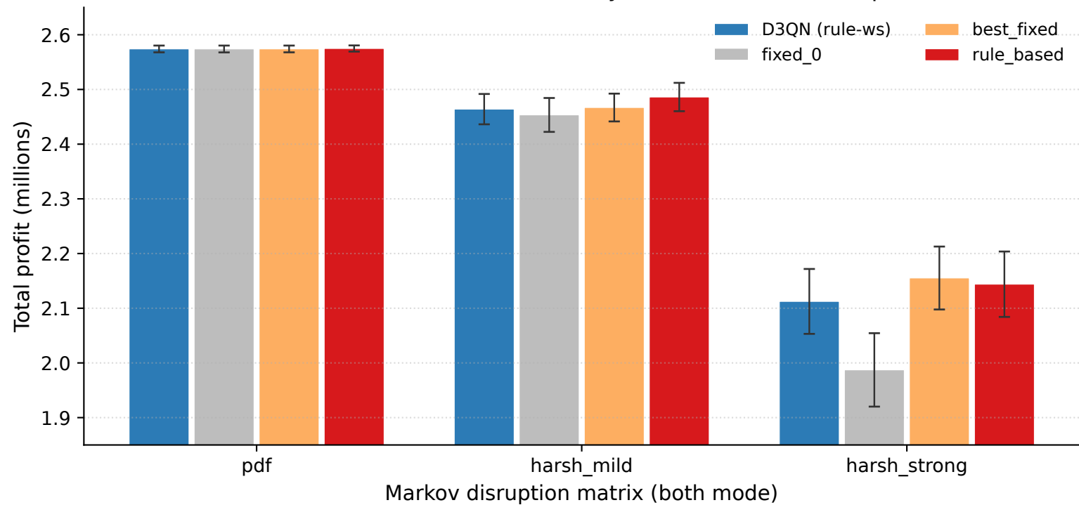
D3QN (rule-ws) vs baselines by matrix (Suite B, 30-rep)
