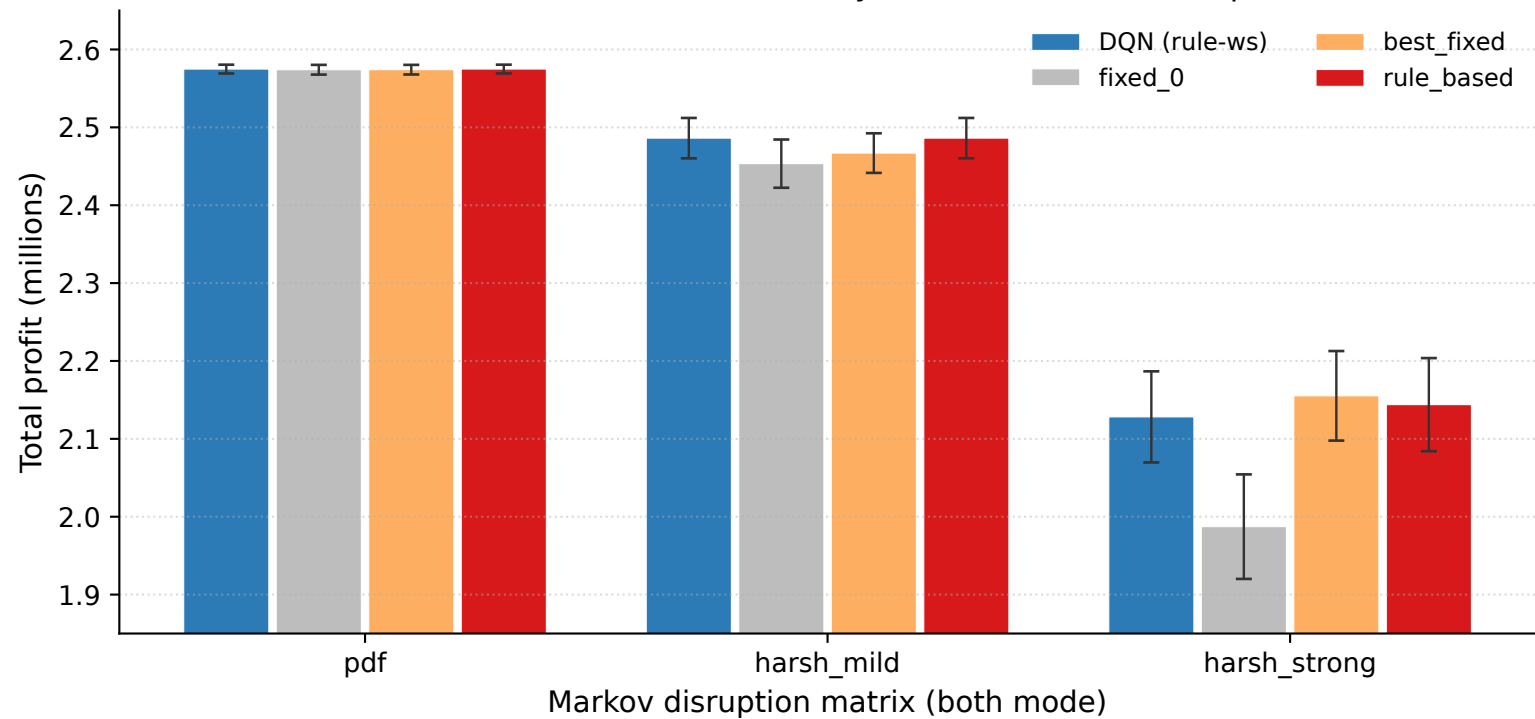
DQN (rule-ws) vs baselines by matrix (Suite B, 30-rep)
