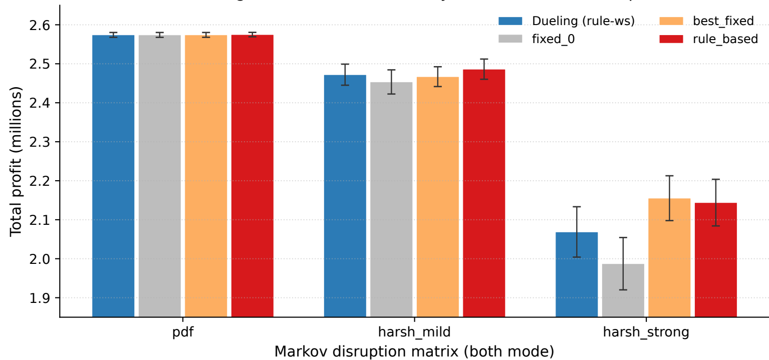
Dueling (rule-ws) vs baselines by matrix (Suite B, 30-rep)
