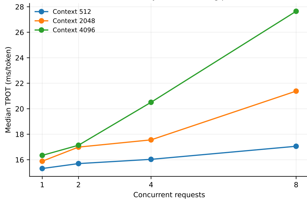
(c) Decode latency under batching pressure
