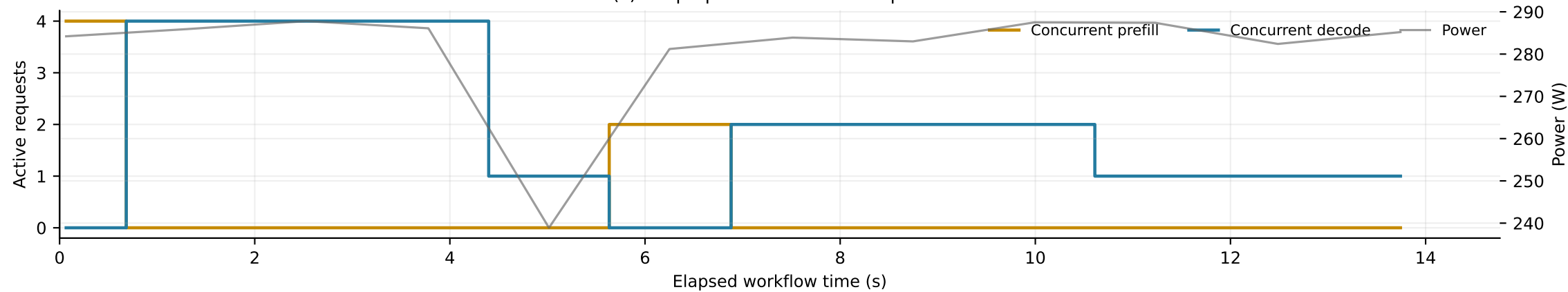
(c) Graph pressure and board power
