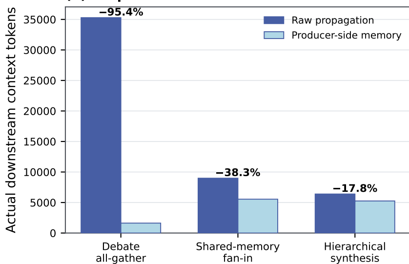
(b) Graph-aware materialization removes retransmission
