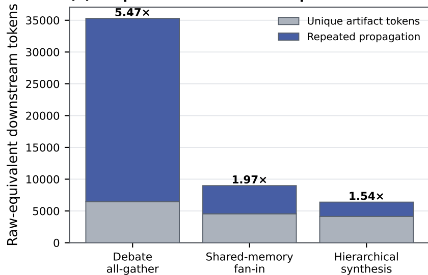
(a) Graph-induced context amplification
