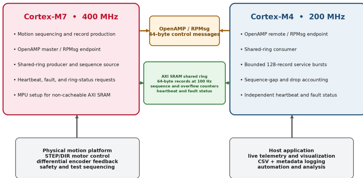
Figure 1. Dual-core architecture: OpenAMP/RPMsg control plane and AXI-SRAM high-rate data plane.
