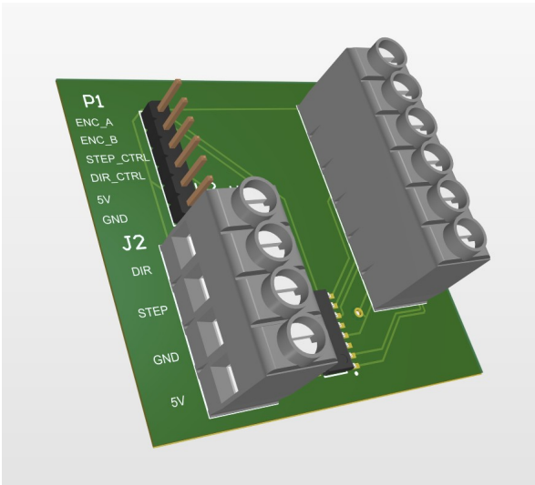
Figure 6. Populated PCB assembly render.
