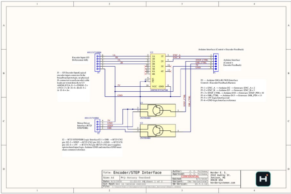
Figure 5. Encoder and STEP/DIR interface schematic.
