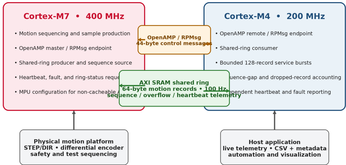
Figure 2. STM32H747 architecture separating low-rate OpenAMP/RPMsg coordination from the AXI-SRAM motion-data path.
