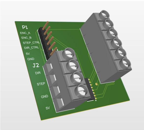
Figure 2. Populated interface PCB.
