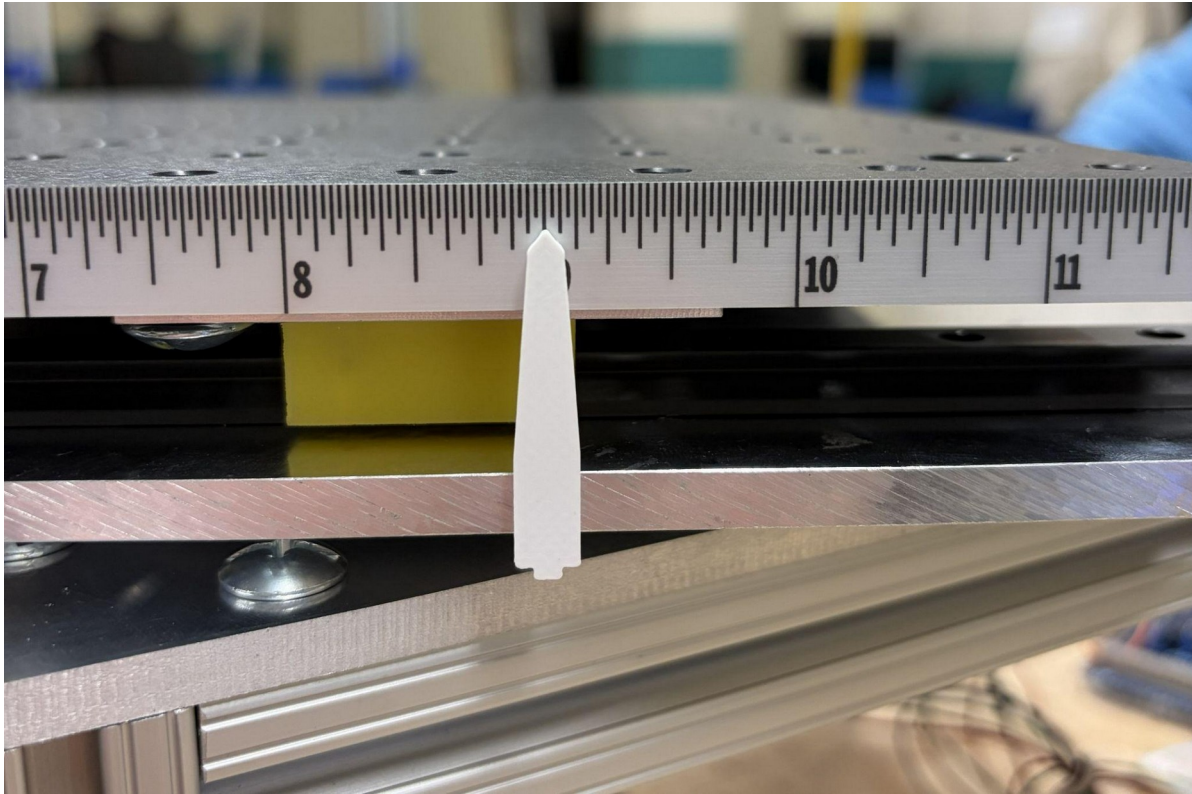
Figure 3. Translation reference near a centered/measured stage position.
