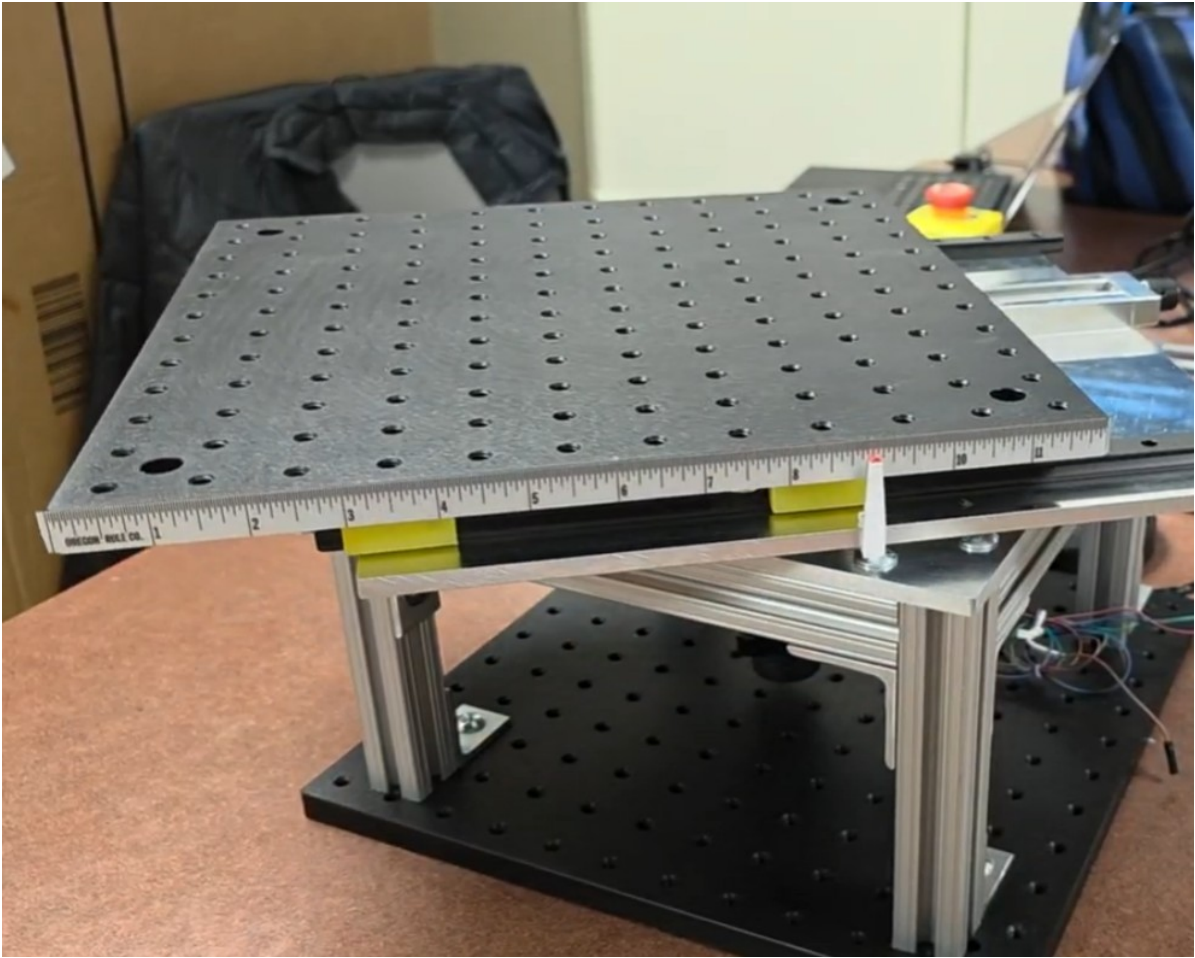
Figure 1. Completed motion platform; the photograph is cropped to keep the public evidence focused on the test article.
