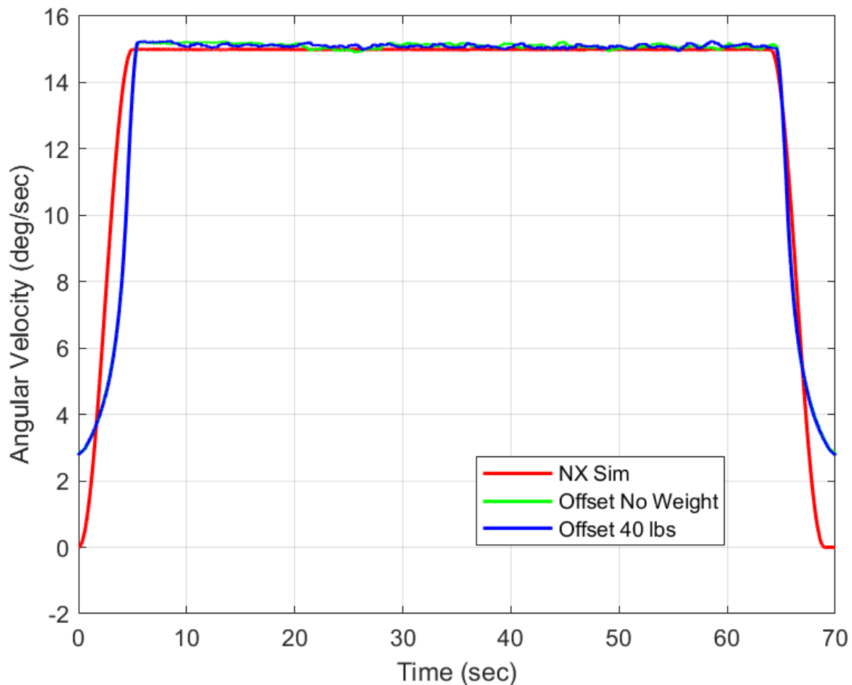
Figure 6. Representative integrated-platform rotational response under test.
