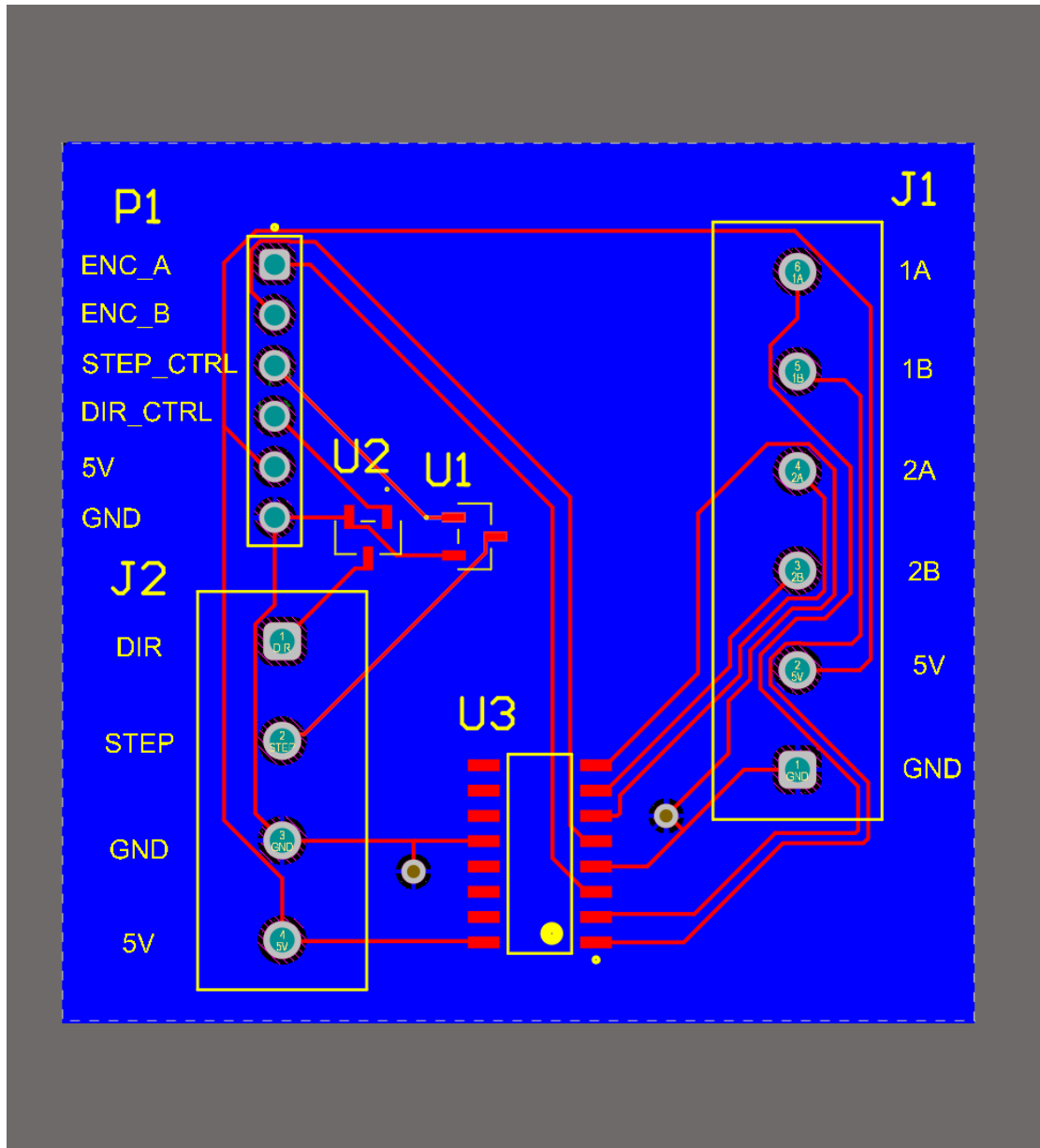
Figure 6. Routed signal and power layer.
