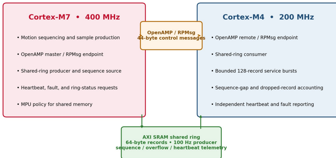
Figure 1. Dual-core STM32H747 architecture separating motion-control responsibilities from inter-core service and telemetry work.
