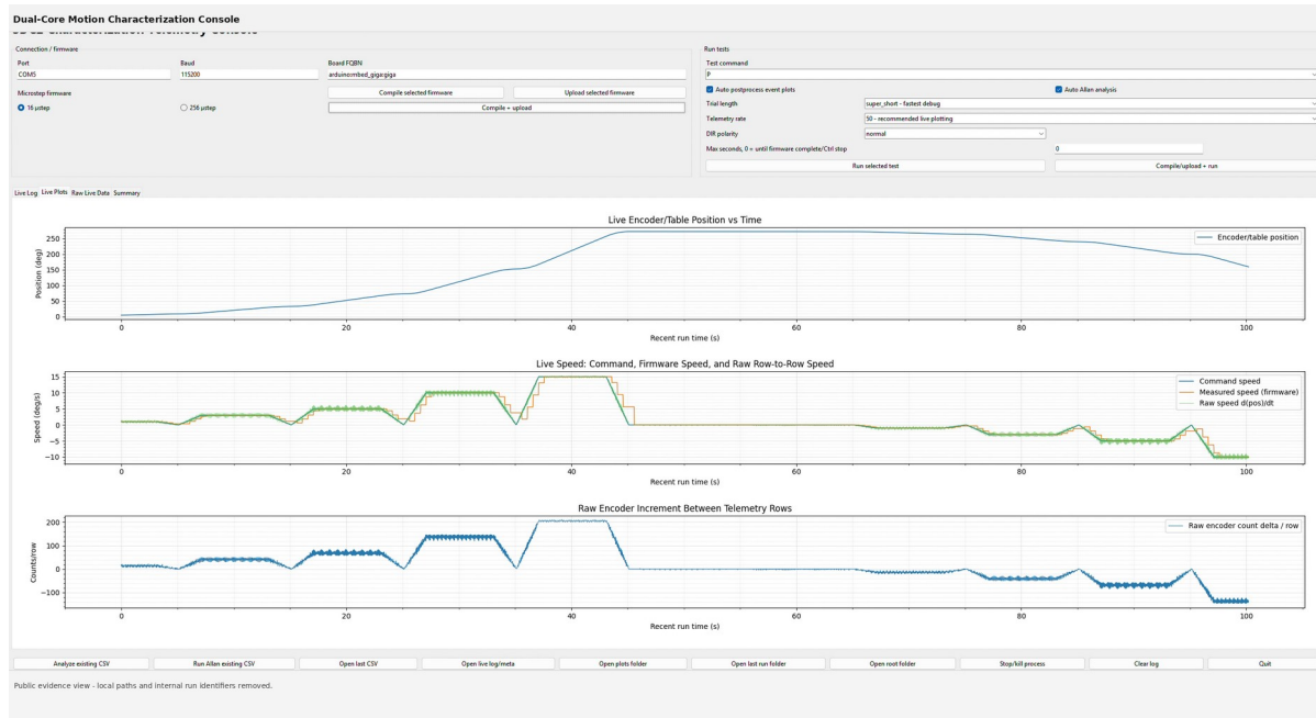
Figure 3. Host console view showing live encoder position, commanded and measured speed, and raw encoder increments.
