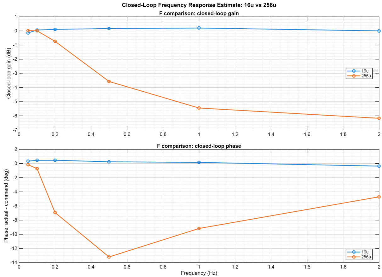
Figure 7. Closed-loop response estimate across the tested frequency range.
