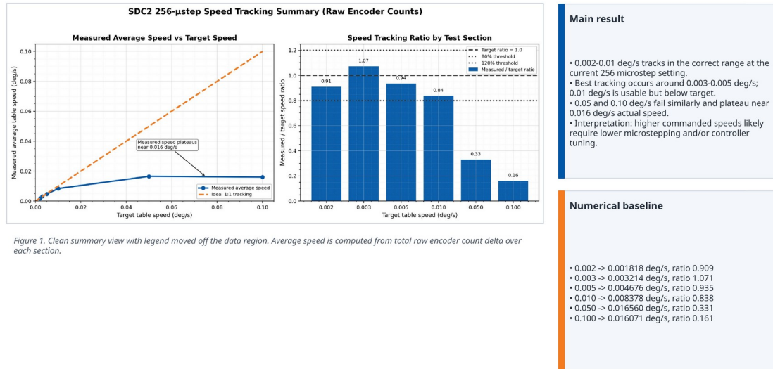
Figure 4. Speed-tracking summary across the characterized low-speed operating range and observed high-speed ceiling.
