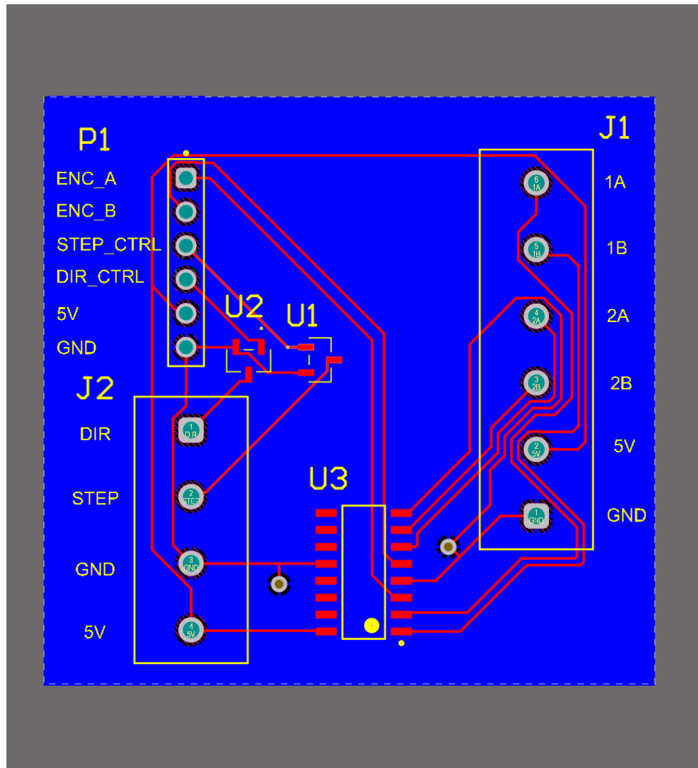
Figure 9. Routed signal layer showing component placement and connector organization.
