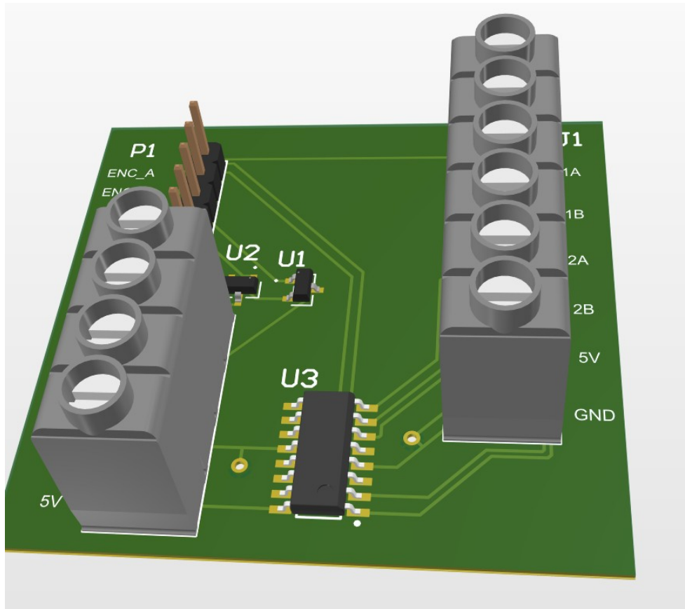
Figure 11. Angled PCB assembly rendering showing the prototype connector and receiver arrangement.
