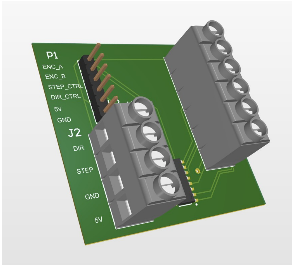
Figure 7. Populated 3D rendering of the custom encoder and STEP/DIR interface PCB.
