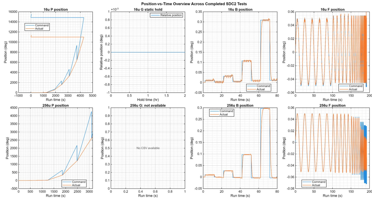
Figure 8. Representative scripted test sequences generated and recorded through the target/host workflow.
