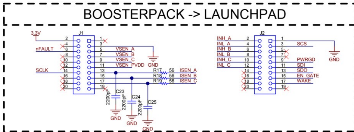
Figure 8. BoosterPack-to-LaunchPad interface reference used during hardware integration.
