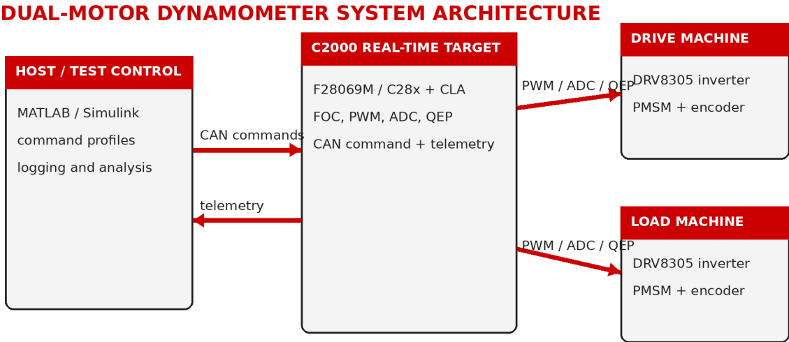
Figure 1. Public functional architecture and system boundary.
