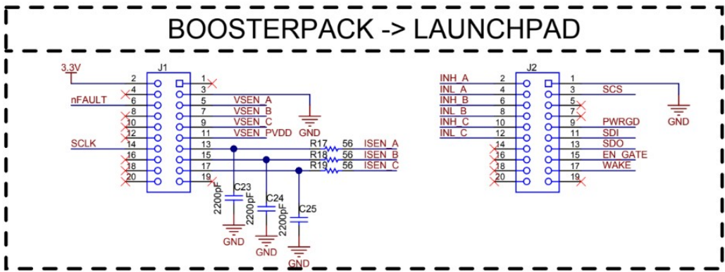
Figure 2. BoosterPack-to-LaunchPad board-interface reference retained with the release.
