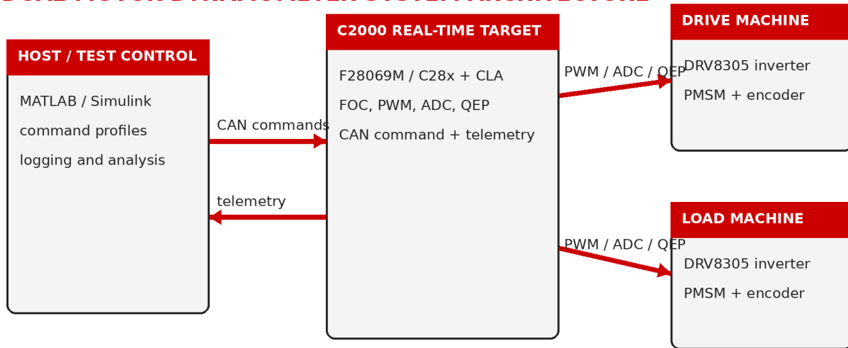
Figure 1. Public system architecture and responsibility boundary.
