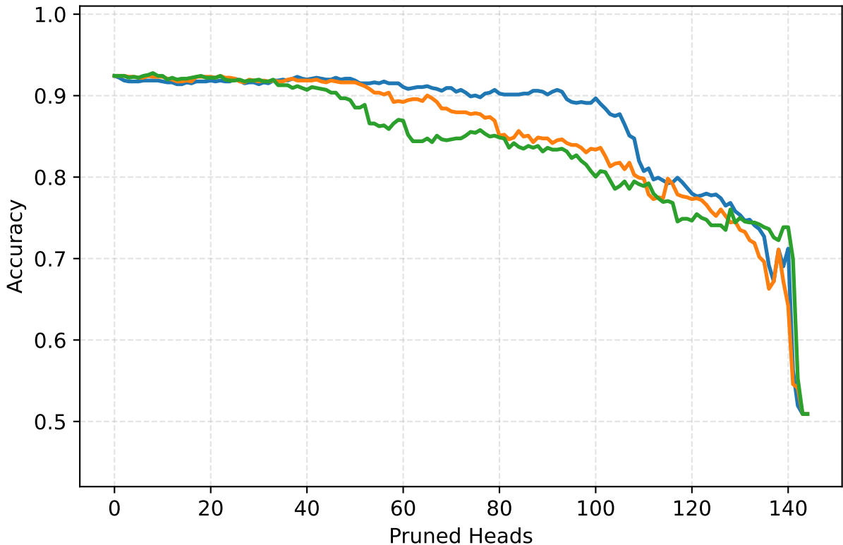
BERT - SST-2: Greedy-Gnorm Variants Comparison
