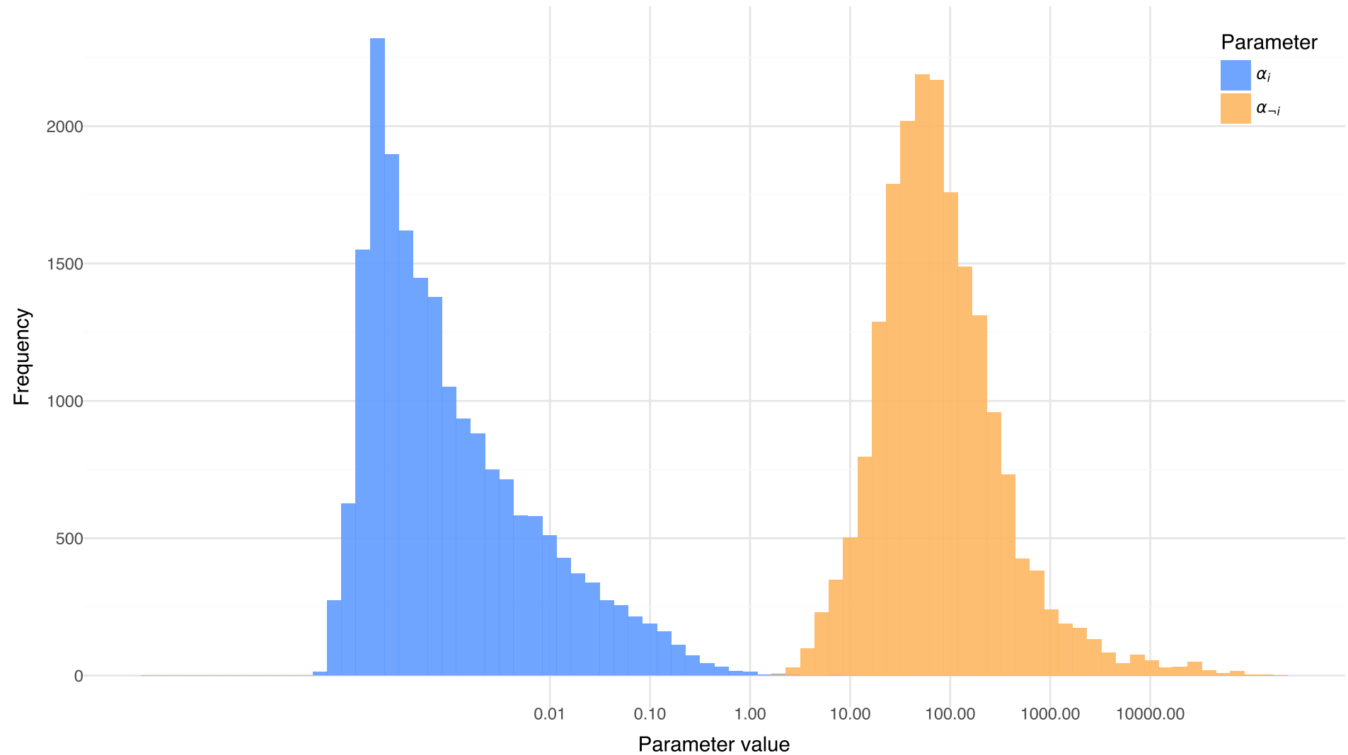
Empirical distributions of \alpha_i and \alpha_{\neg i}
