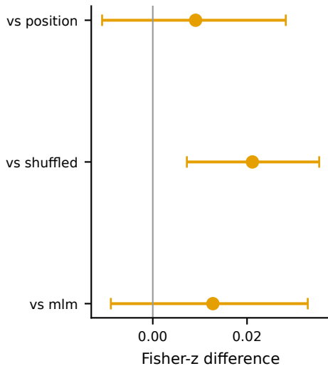
ZuCo transfer: mean and 95% CI
