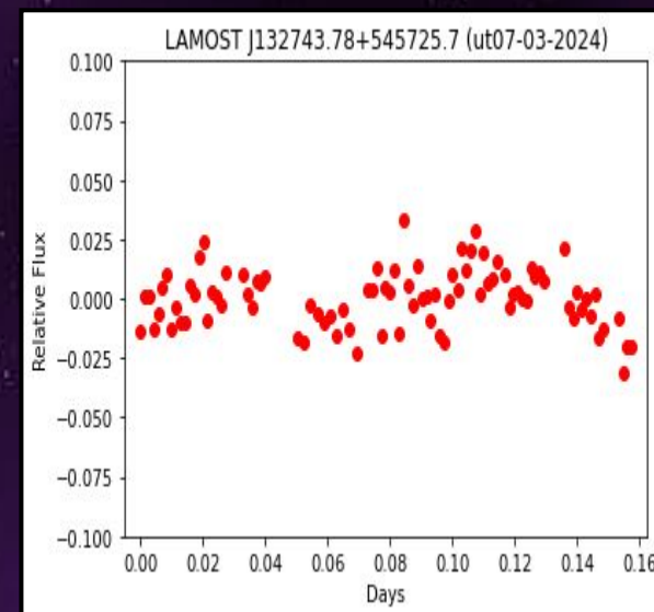
Normalized light curve of J1327 (UT July 3rd, 2024)
