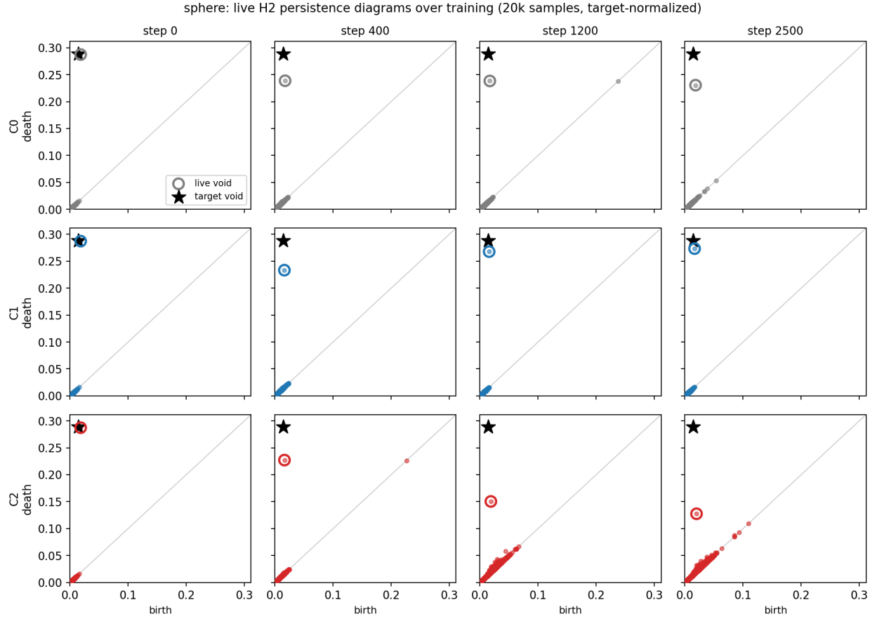
Figure 6: Live H2 persistence diagrams over training (one sphere seed; 20k samples, target-normalized; star = target void bar, circle = most persistent live bar). Top , baseline: the void drifts off target. Middle , loss: the void returns to the target once the ramp activates. Bottom , repulsion control: the void is pinned and dragged away while near-diagonal phantom bars accumulate.
