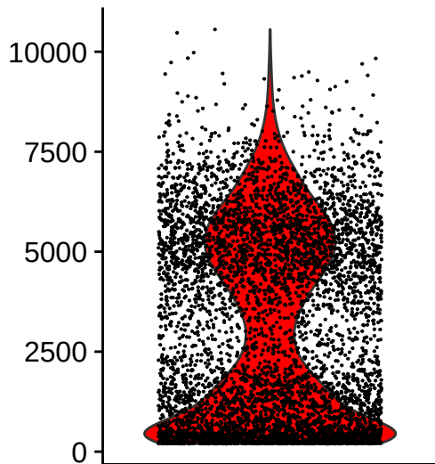
nFeature_RNA
