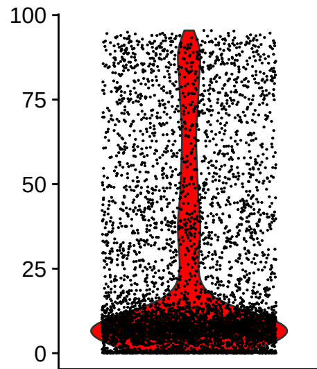
percent.mt
