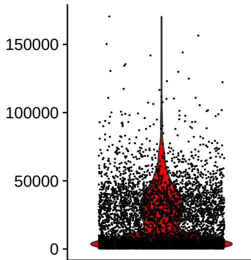
nCount_RNA
