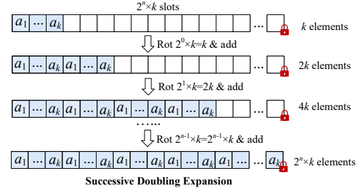
Fig. 3. Successive doubling expansion for matrix A when computing matrix multiplication A \times B , where A \in \mathbb{R}^{m \times n} and B \in \mathbb{R}^{n \times k} .
