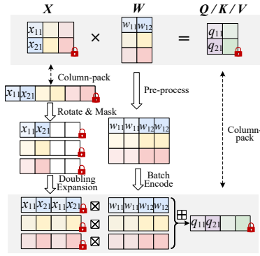
Fig. 4. A toy example of SIMD encoding in Ct-Pt matrix multiplication, where X \in \mathbb{R}^{2 \times 3} and the weight matrix W \in \mathbb{R}^{3 \times 2} .
