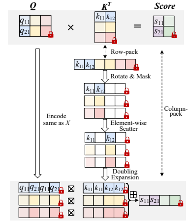
Fig. 6. A toy example of SIMD encoding in Q \times K^T , where Q \in \mathbb{R}^{2 \times 3} and K^T \in \mathbb{R}^{3 \times 2} .
