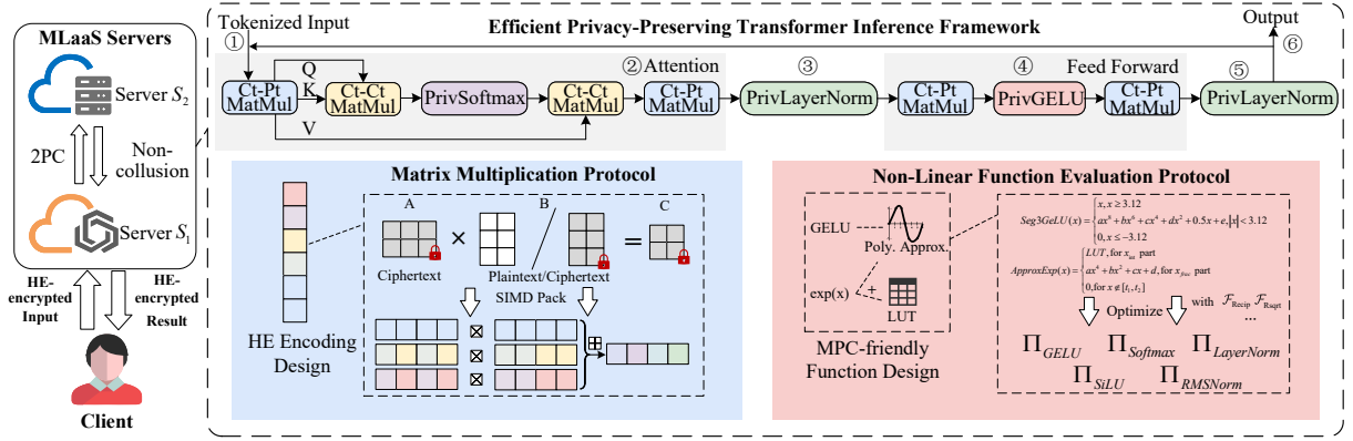
Fig. 2. Overview of PrivTI. The framework consists of our proposed HE-based matrix multiplication protocol and MPC-based non-linear function evaluation protocol to enable efficient privacy-preserving inference for transformer-based models.
