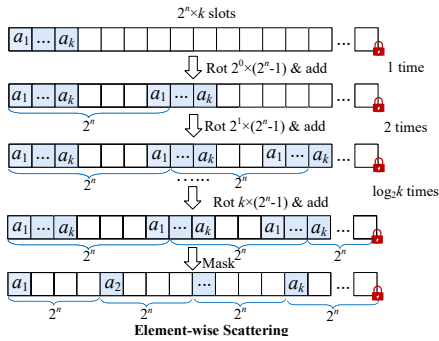
Fig. 5. Element-wise scattering for matrix A when computing the matrix multiplication A \times B , where A \in \mathbb{R}^{m \times n} and B \in \mathbb{R}^{n \times k} .
