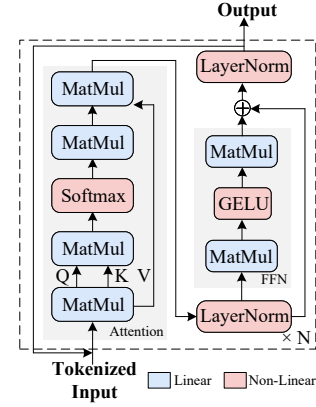
Fig. 1. Transformer Architecture.
