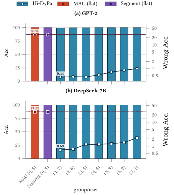
Figure 5: Collusion resistance against three-colluder attacks across group/user splits (L_g, L_u) with L_g + L_u = 8 , the flat baselines MAU [9] and Segment [43] being the (0, 8) case.
