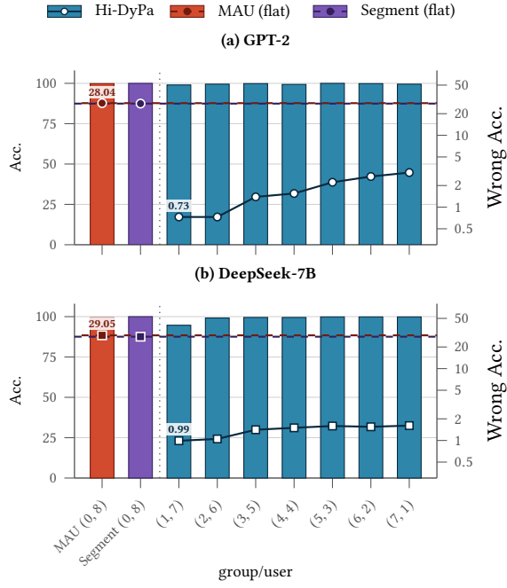
Figure 4: Collusion resistance against two-colluder attacks across group/user splits, the flat baselines MAU [9] and Segment [43] being the (0, 8) case.
