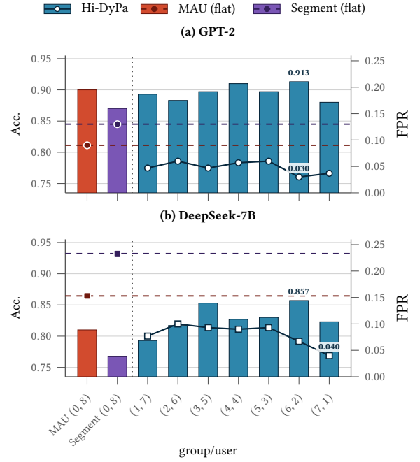
Figure 3: Clean-text detection across group/user splits (L_g, L_u) with L_g + L_u = 8 , the flat baselines MAU [9] and Segment [43] being the (0, 8) case.
