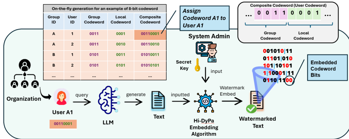
Figure 1: Hi-DyPa scheme: Watermark Generation, Embedding Stage and Key Management.
