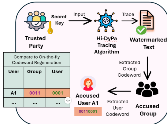
Figure 2: Hi-DyPa scheme: Watermark detecting and tracing. All the extracted group or user codewords are compared to the on-the-fly codeword generation. The trusted parties can access the watermarking secret key from the system admin if they are authorized to trace the LLM-misuse users.
