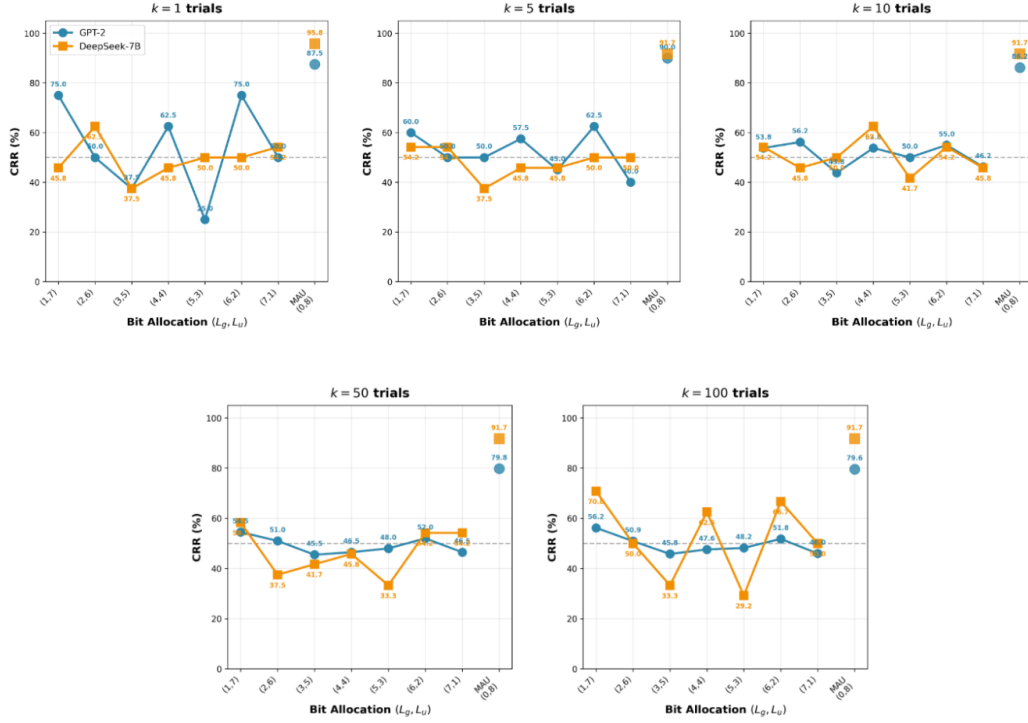
Figure 6: Codeword Recovery Rate (CRR) across different adversarial colluding trials
