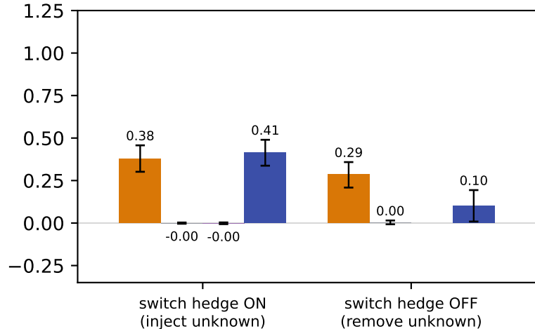
entropy recovery
