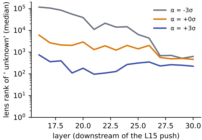
steering the direction on known twins
