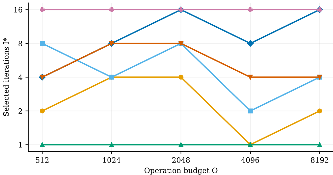
Selected iterations I^* by operation budget
