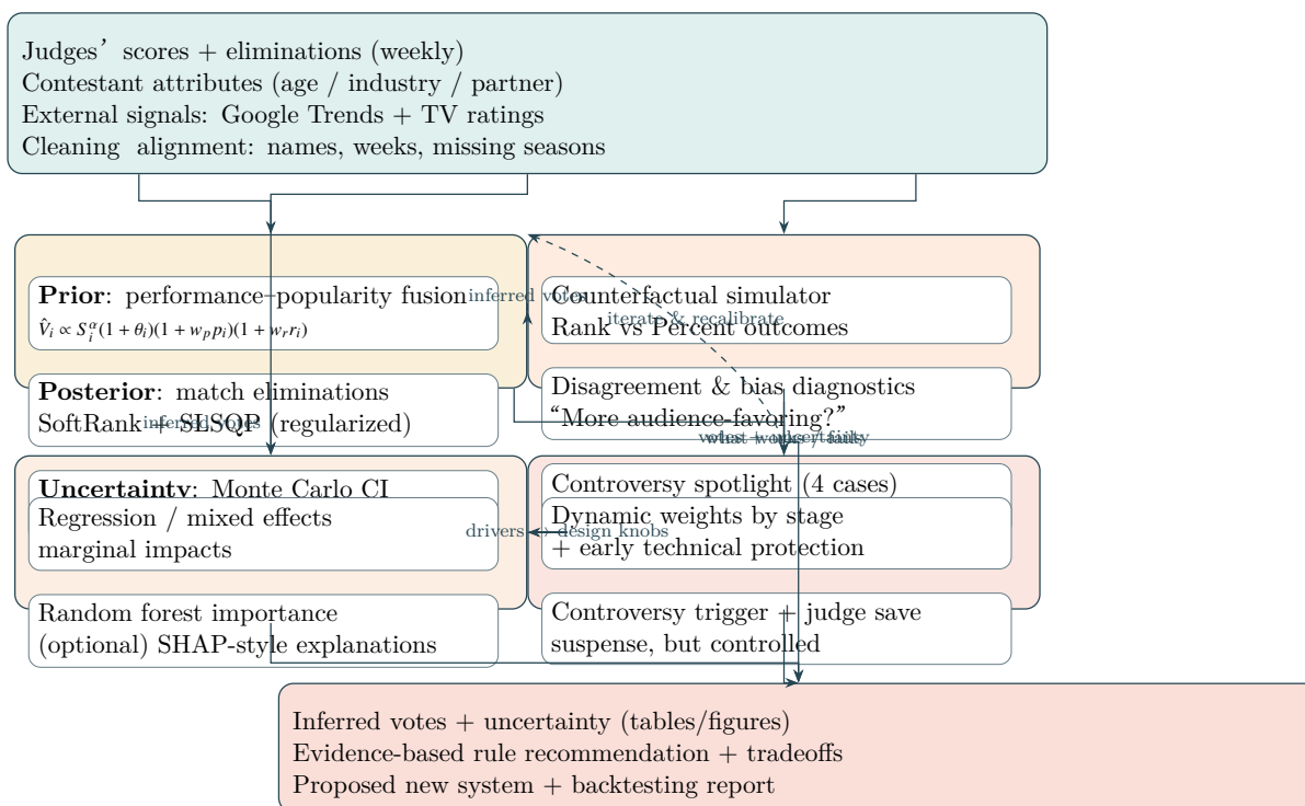
Figure 1: Our four-task workflow with explicit interactions: Task 1 infers hidden audience votes under real elimination constraints; Tasks 2–3 analyze rule effects and preference drivers; Task 4 synthesizes evidence into a new system and backtests it with a scorecard.
