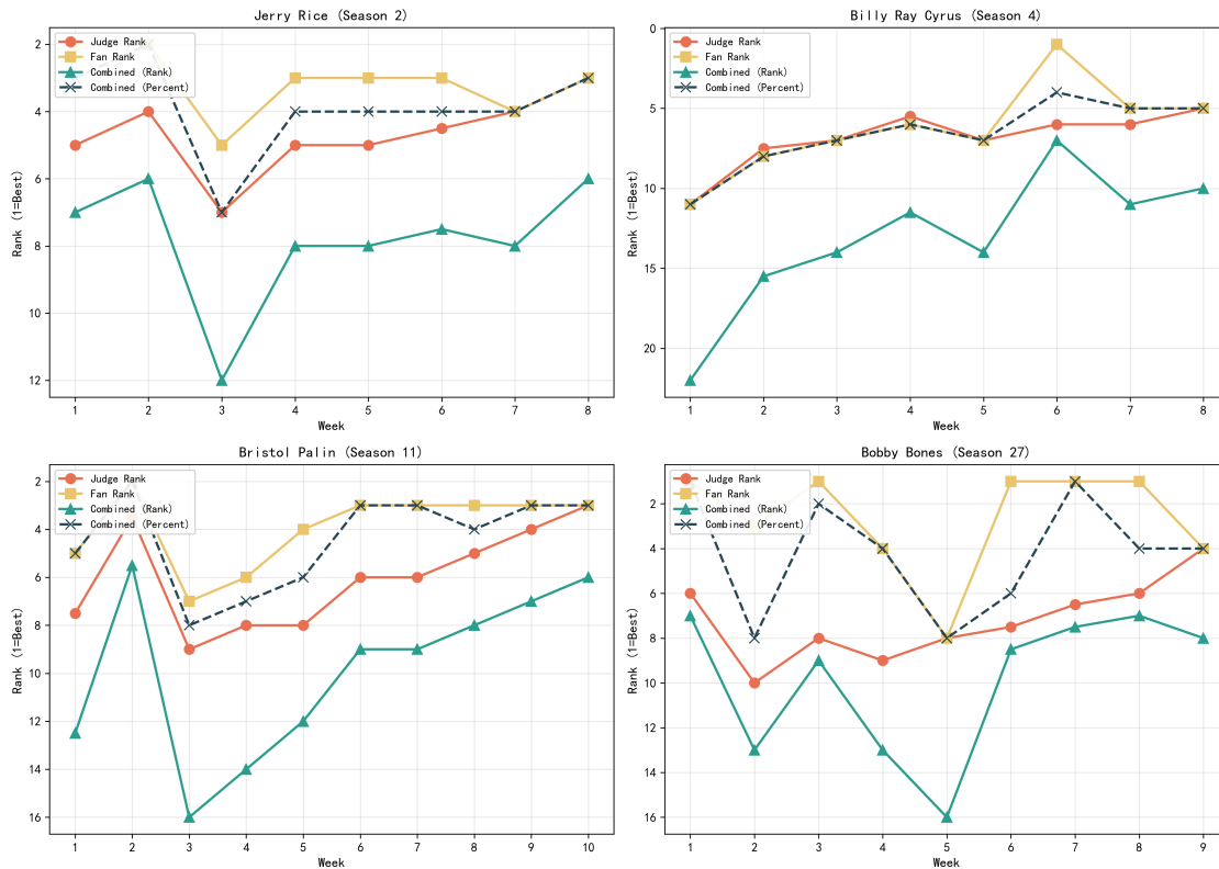
Figure 7: Weekly Trajectories of Four Controversial Contestants
