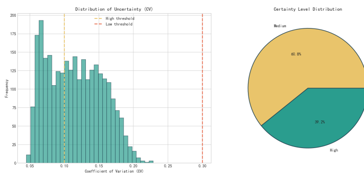
Figure 5: Uncertainty Distribution: 39.2% High Certainty, 60.8% Moderate Certainty, with Contestant/Week Variation.
